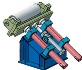
SNUBBER ROLL
