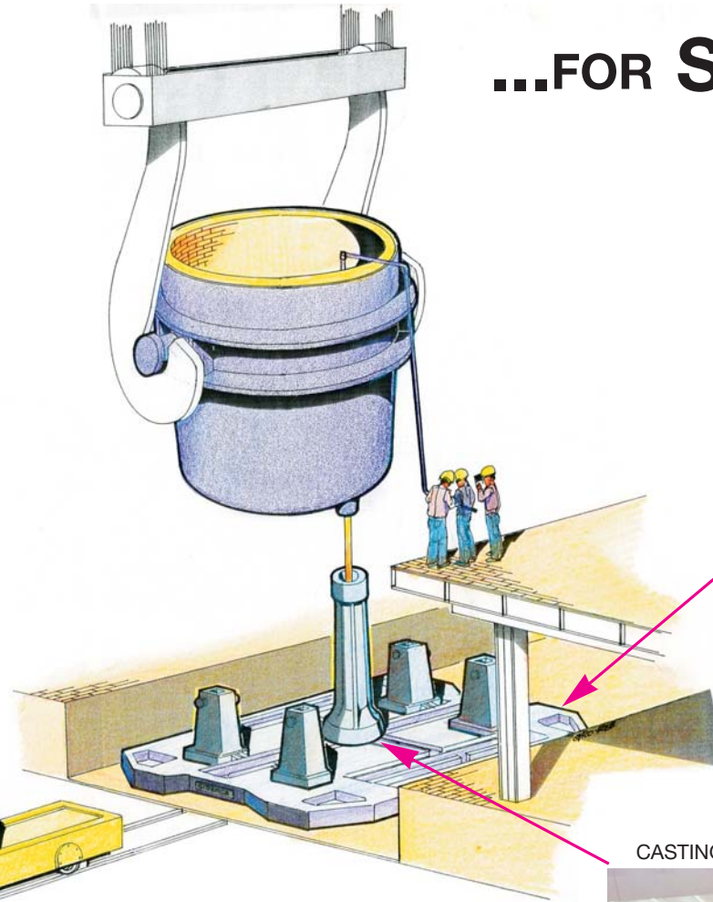
POLYGONAL MOULDS FOR STEEL FORGING
