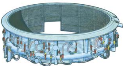
WATER-COOLED E.A.F. WALL & VAULT
